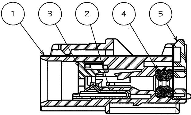
SECT. A-A
