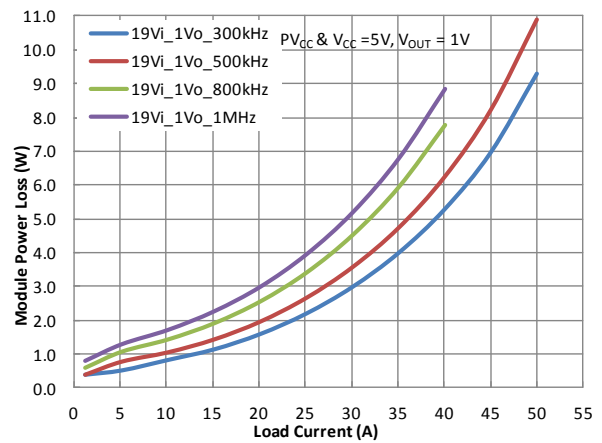
Figure 7. Power Loss vs. Output Current with 19 V IN
