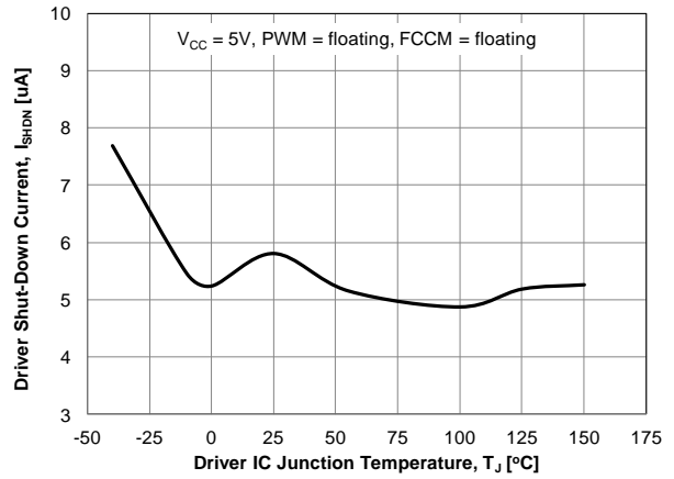
Figure 22. Driver Shutdown Current vs. Temperature
