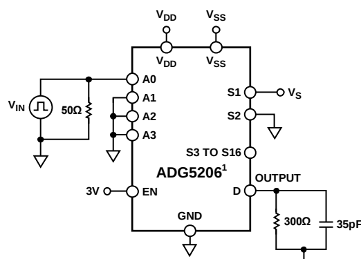
Figure 35. Address to Output Switching Times, t_{TRANSITION}
