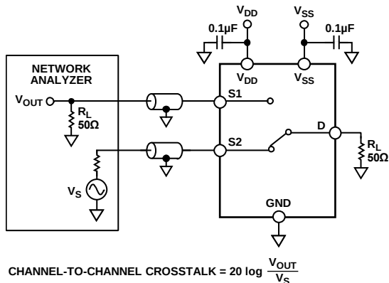
Figure 40. Channel-to-Channel Crosstalk
