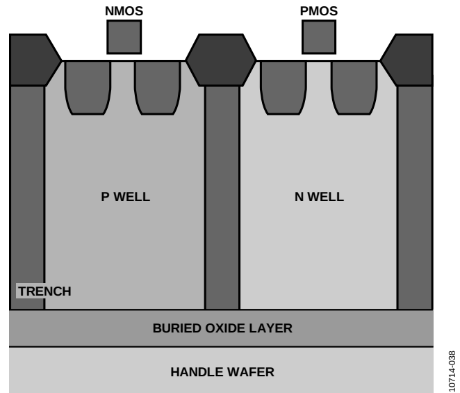
Figure 42. Trench Isolation
