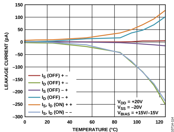
Figure 16. Leakage Currents vs. Temperature, \pm 20 V Dual Supply
