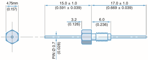
M4 x 0.7 - 6g Thread 4.75mm Hexagonal Head
