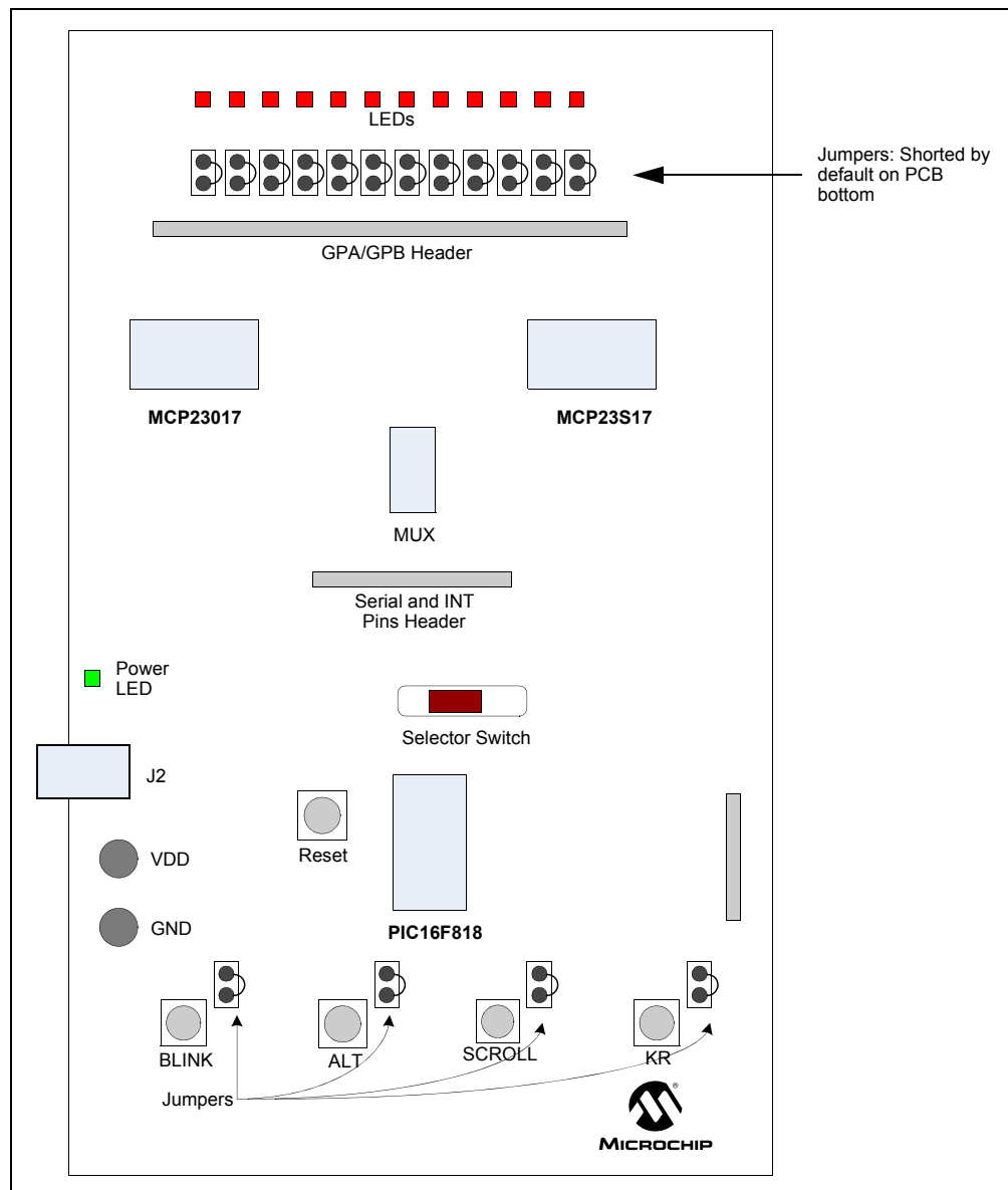
FIGURE 2-1: BOARD LAYOUT
