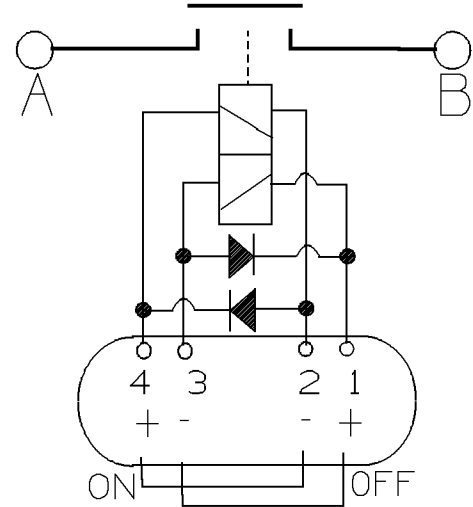
Pin Assignment
