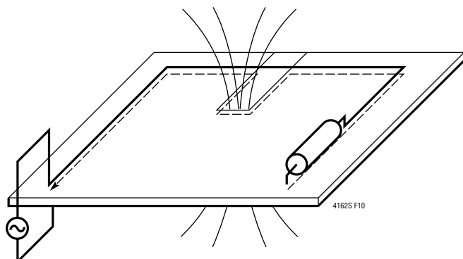
Figure 10. Currents Tend to Follow Their Natural Least Area Path. Breaks in the Ground Plane Lead to Increased Impedance and EMI
