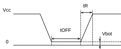
Figure 58. Rise waveform
