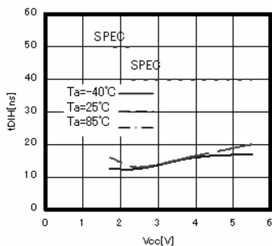
Figure 22. SI hold time t_{DIH}
