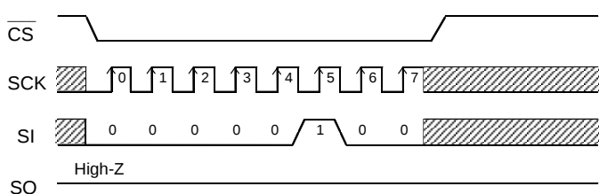
Figure 34. Write disable
