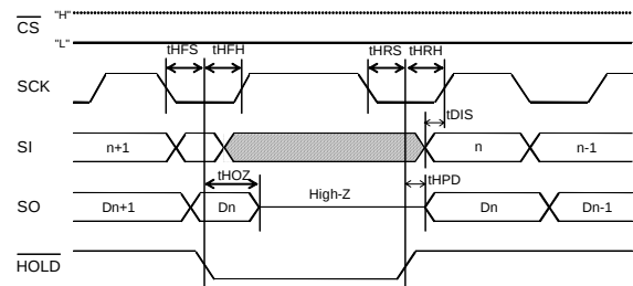
Figure 3. HOLD timing
