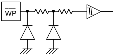
Figure 56. \overline{WP} input equivalent circuit
