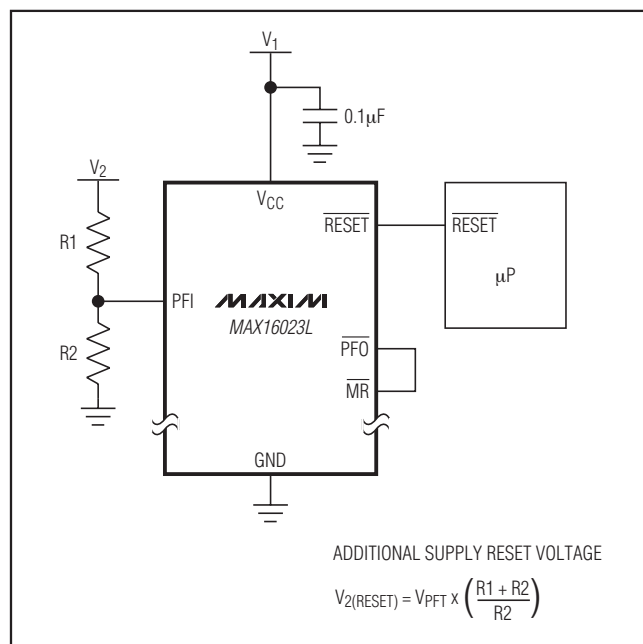
Figure 3. Monitoring an Additional Supply by Connecting \overline{PFO} to \overline{MR}
