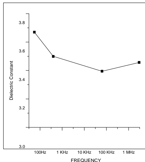
Dielectric Constant Versus Frequency
