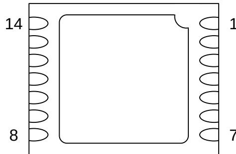
Figure 2: Package pinout (bottom view)
