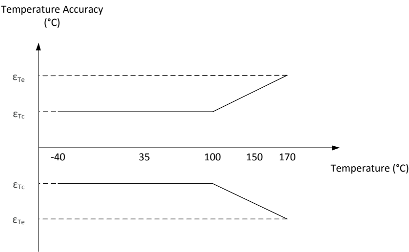
Figure 8: NTC temperature accuracy
