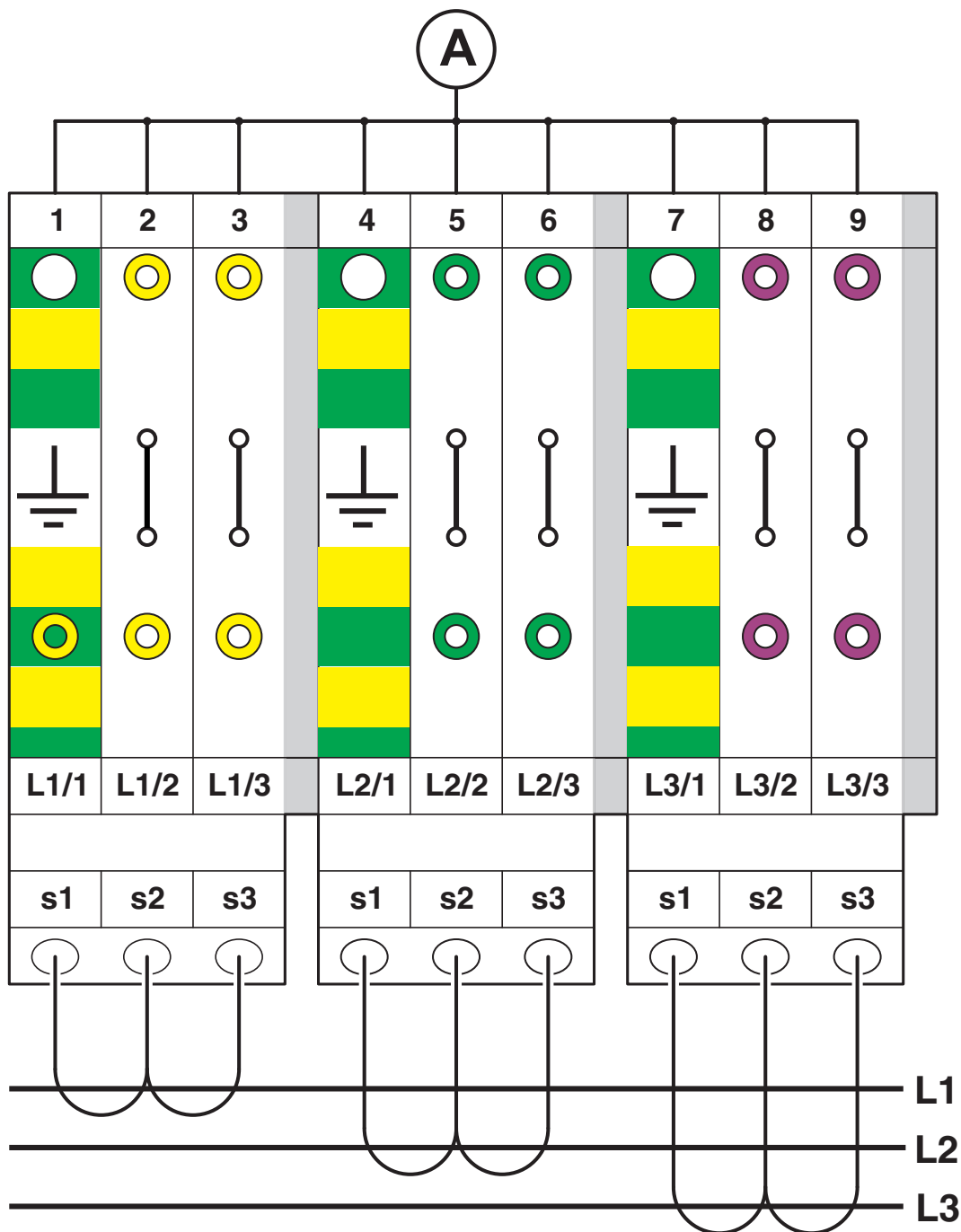
Connection diagram
