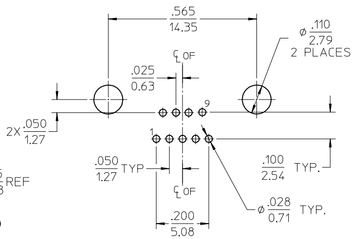
RECOMMENDED P.C.B. LAYOUT SOLDER SIDE
