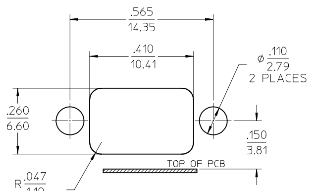
RECOMMENDED PANEL CUT-OUT .055/1.40 MAX PANEL THICKNESS
