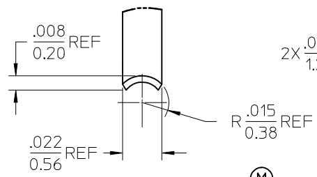
CONTACT PROFILE (M) Detail 1 Scale 20:1
