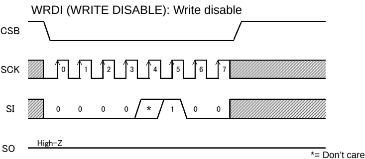
Figure 36. Write disable
