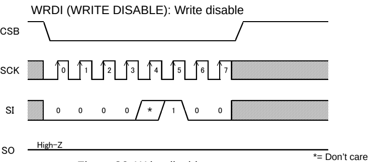
Figure 36. Write disable
