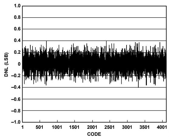
Figure 15. ADC DNL
