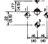
Component Side Layout
