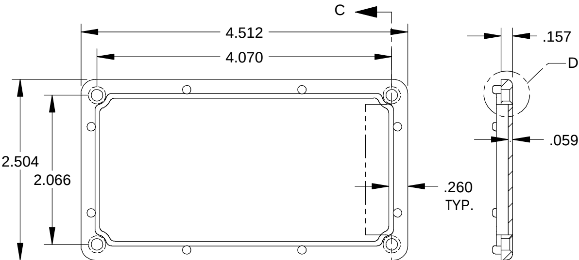
SECTION C-C
