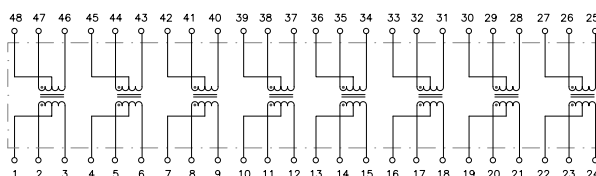
Circuit C
