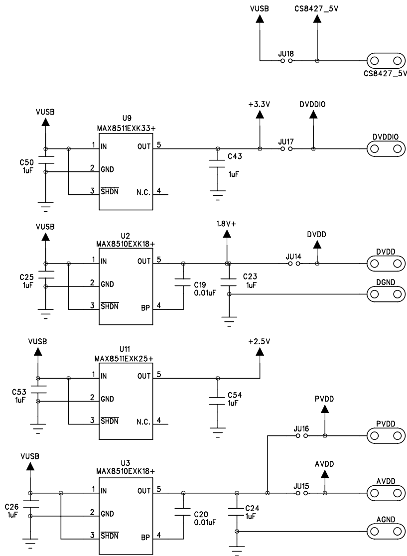
Figure 11d. MAX9867 EV Kit Schematic (Sheet 4 of 4)
