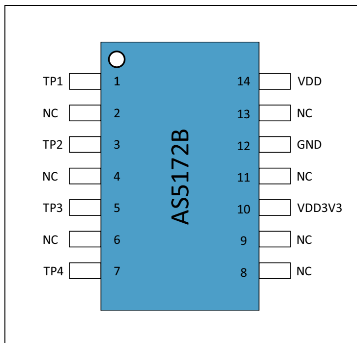
Figure 3: AS5172B Pin Assignment (Top View, TSSOP14)
