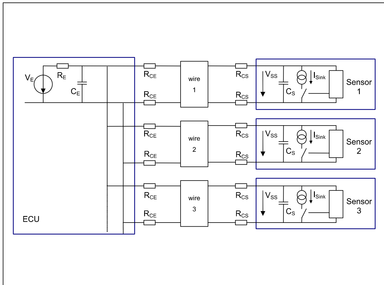
Figure 69: Synchronous Parallel Bus Mode (PSI5-P)
