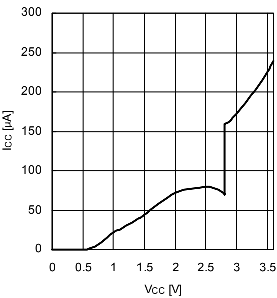
Figure.9 Vcc-Icc
