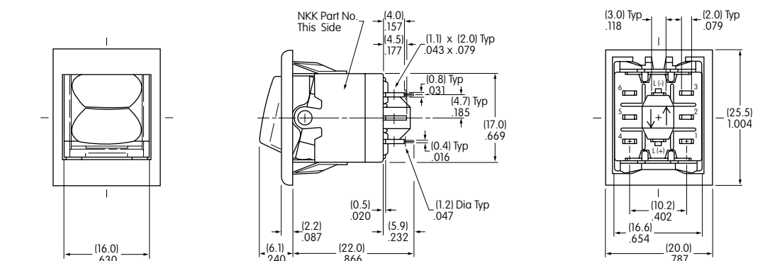
Sculptured Cap Single & Double Pole
