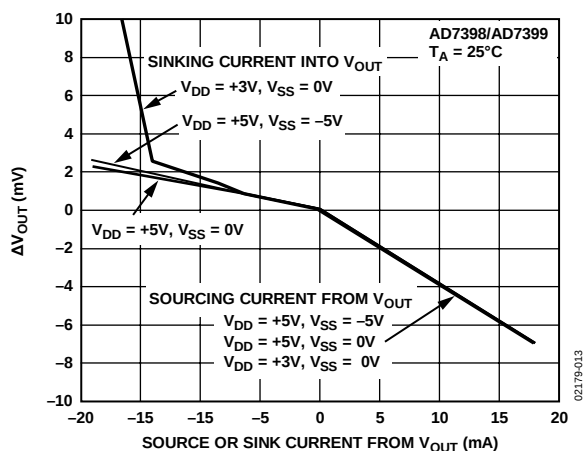
Figure 13. \Delta V_{OUT} vs. Load Current
