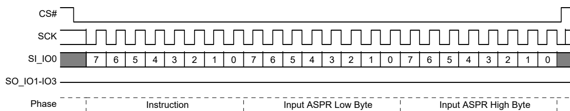
Figure 105. ASPP Command
