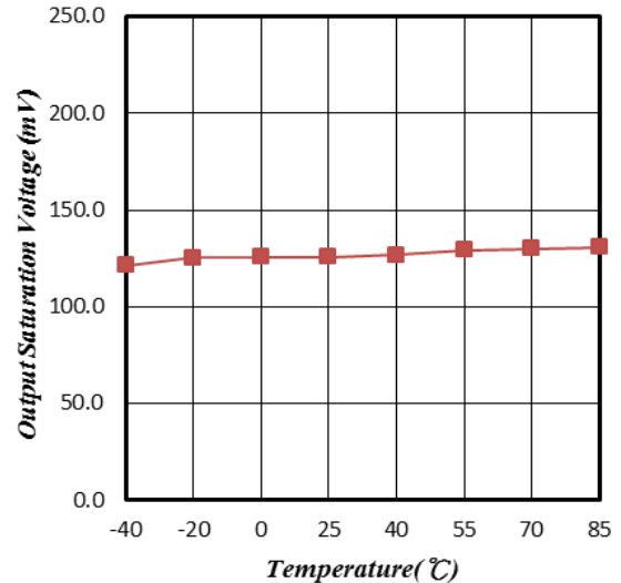
Figure 6. Output Saturation Voltage vs. Temperature
