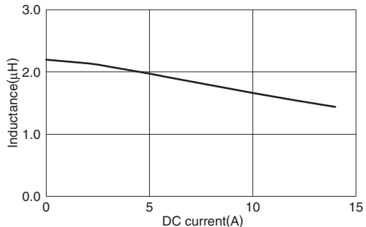
SPM6530T-2R2M
