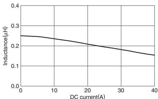
SPM6530T-R25M230
