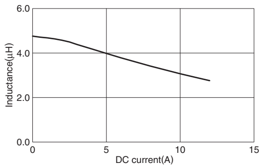
SPM6530T-4R7M
