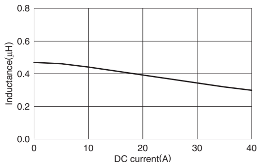
SPM6530T-R47M170
