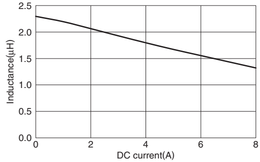
SPM5012T-2R2M
