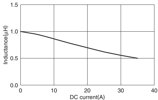
SPM6530T-1R0M120
