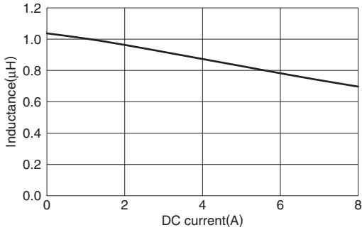
SPM5012T-1R0M
