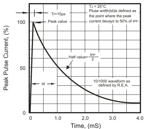
Fig.5 Pulse Waveform
