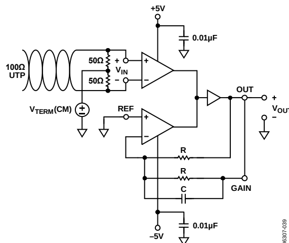
Figure 38. Common-Mode Termination with G = 1
