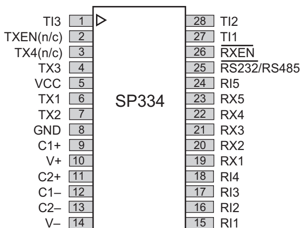
Figure 11. SP334 Pinout
