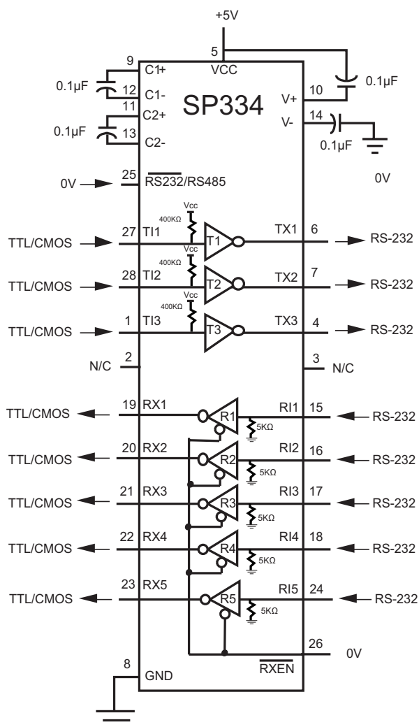
Figure 12. Typical Operating Circuits
