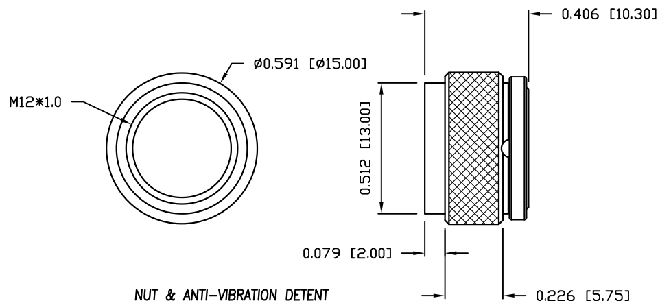
NUT & ANTI-VIBRATION DETENT
