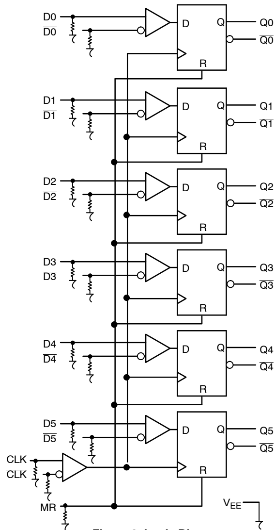
Figure 3. Logic Diagram
