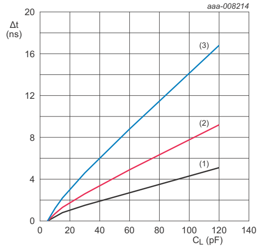
T_{amb} = -40\text{ }^\circ\text{C} to +85\text{ }^\circ\text{C} unless otherwise specified. (1) Minimum: V_{CC} = 1.3\text{ V} (2) Typical: T_{amb} = 25\text{ }^\circ\text{C} ; V_{CC} = 1.2\text{ V} (3) Maximum: V_{CC} = 1.1\text{ V}
