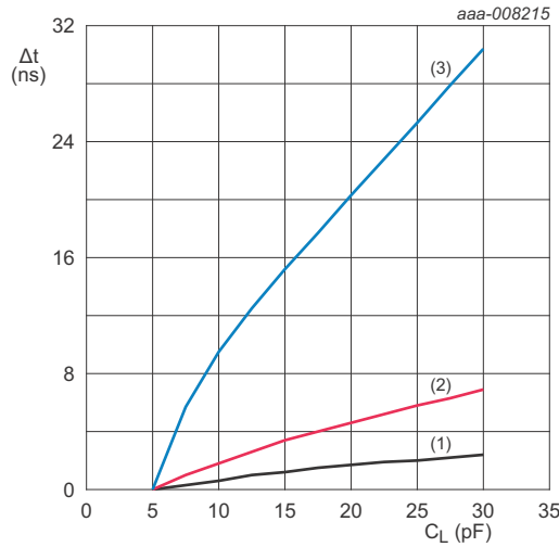
T_{amb} = -40\text{ }^\circ\text{C} to +85\text{ }^\circ\text{C} unless otherwise specified. (1) Minimum: V_{CC} = 0.85\text{ V} (2) Typical: T_{amb} = 25\text{ }^\circ\text{C} ; V_{CC} = 0.8\text{ V} (3) Maximum: V_{CC} = 0.75\text{ V}
