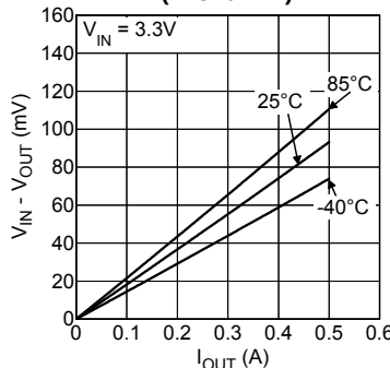
V_{\text{DROP}} vs. Temperature (MIC20XXA)
