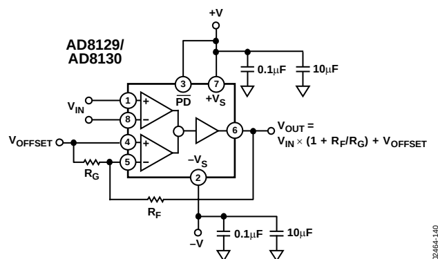
Figure 139. In this Circuit, V_{OFFSET} Appears at the Output with Unity Gain. This Circuit Works Well if the V_{OFFSET} Source Impedance Is Low.
