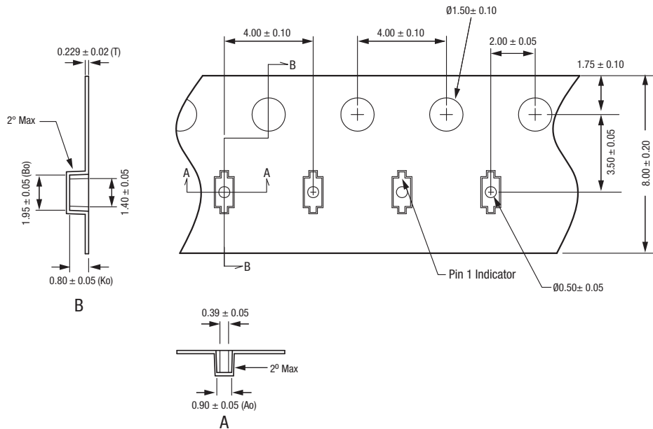
Figure 5. SC-79 Package Dimension Drawing
