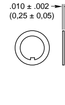
Keyed Washer
