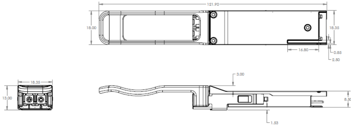
Figure 2 – FTL4C3QE1C mechanical drawing.
