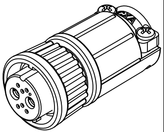
STD COUPLING RING P/N: W3B80-8SG-5XX
