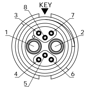
WIRE VIEW
