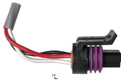
Metri-Pack 150 mating connector 2
