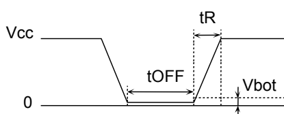
Figure 65. Rise Waveform
