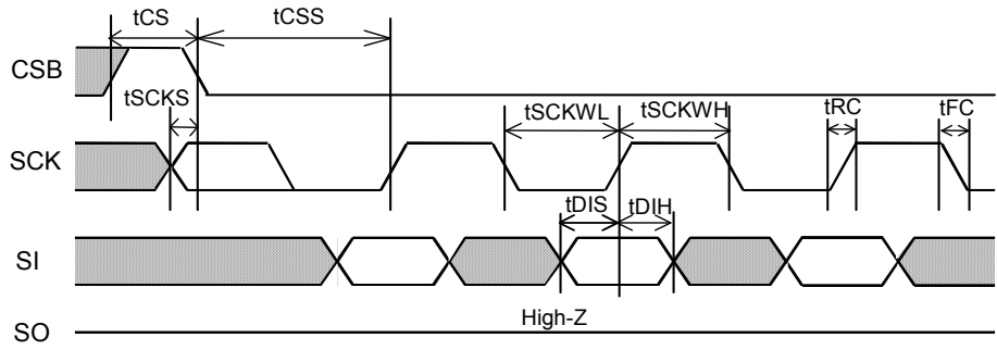
Figure 2. Input Timing
