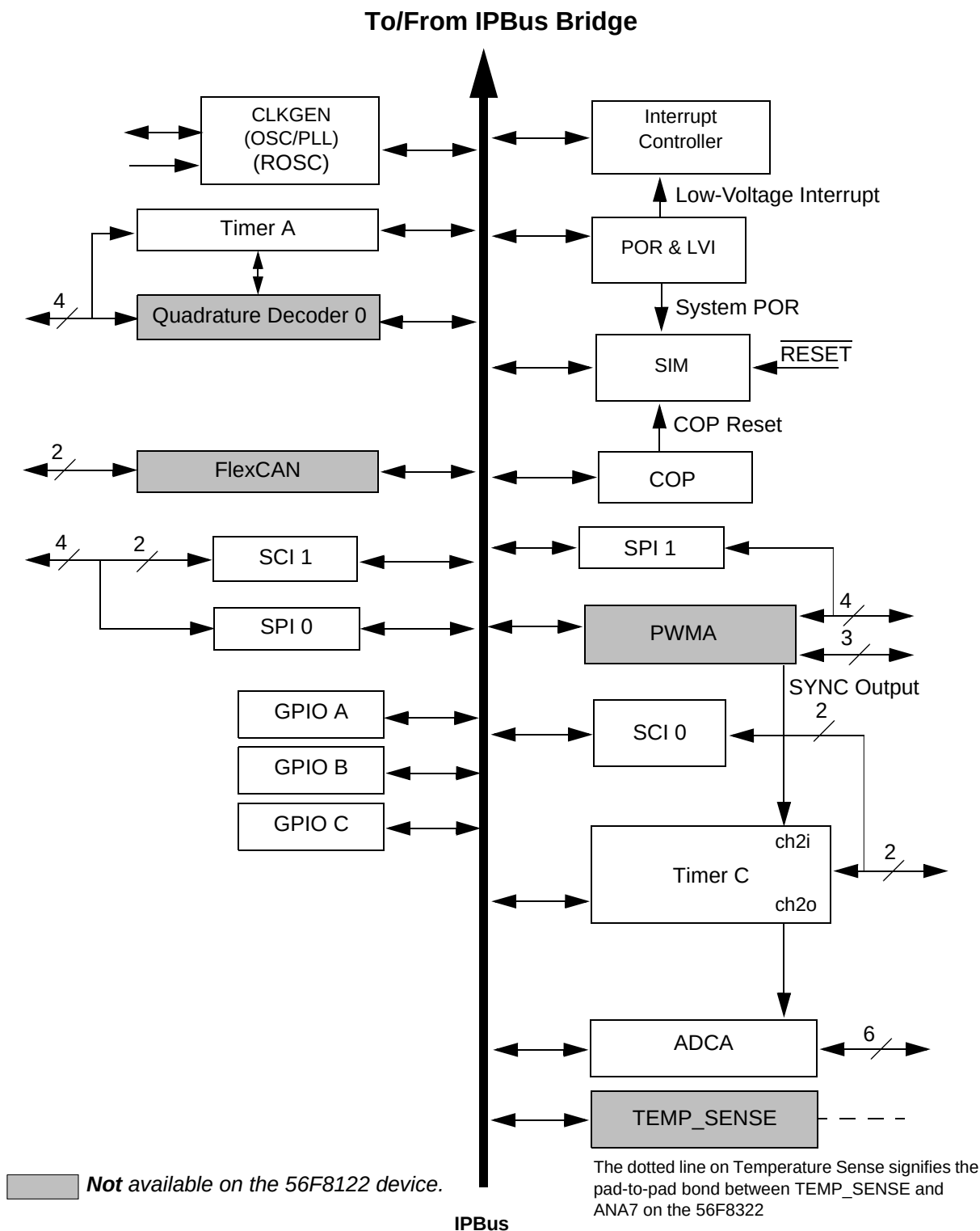
Figure 1-2 Peripheral Subsystem
