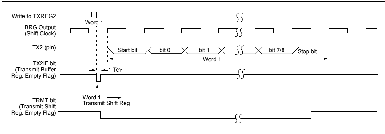
FIGURE 19-2: ASYNCHRONOUS TRANSMISSION
