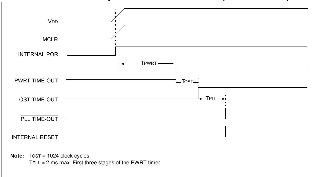
FIGURE 5-7: TIME-OUT SEQUENCE ON POR W/PLL ENABLED ( \overline{\text{MCLR}} TIED TO V_{DD} )
