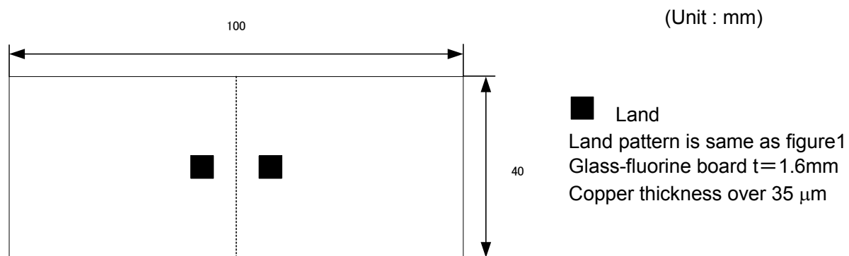
Fig. 2 Testing board
