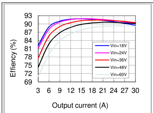
Figure 9: AVO100-36S3V3B-6L Efficiency Curves @ 25 degC
