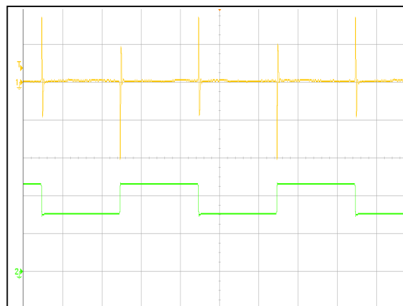
Figure 8: AVO100-36S3V3B-6L Transient Response (2mS/div) 50%~75%~50% load change, 1A/uS slew rate, Ch 1: Vo (100mV/div) Ch 2: Io (10A/div)
