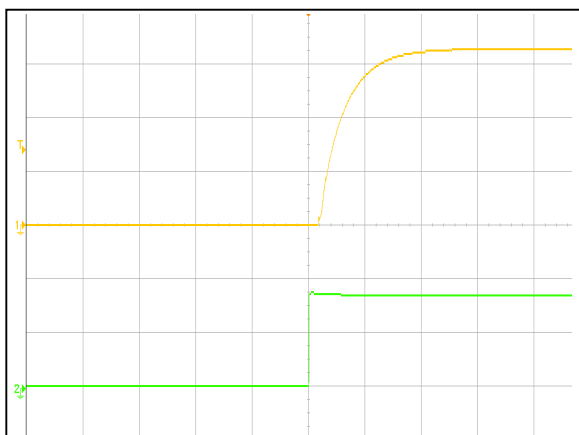
Figure 3: AVO100-36S3V3B-6L Output Voltage Startup Characteristic
