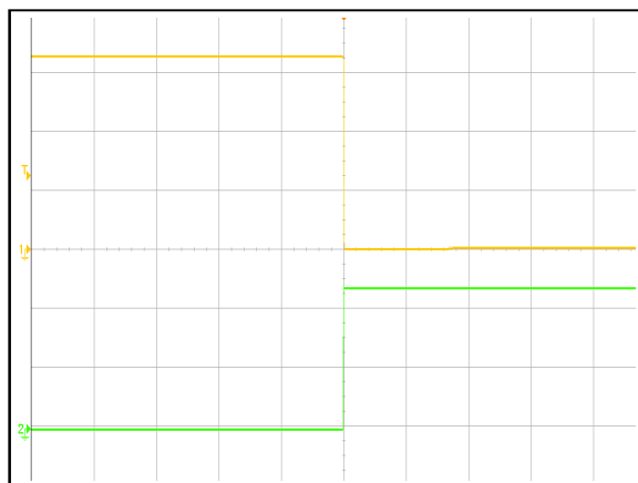
Figure 6: AVO100-36S3V3B-6L Remote OFF Waveform (50ms/div)
