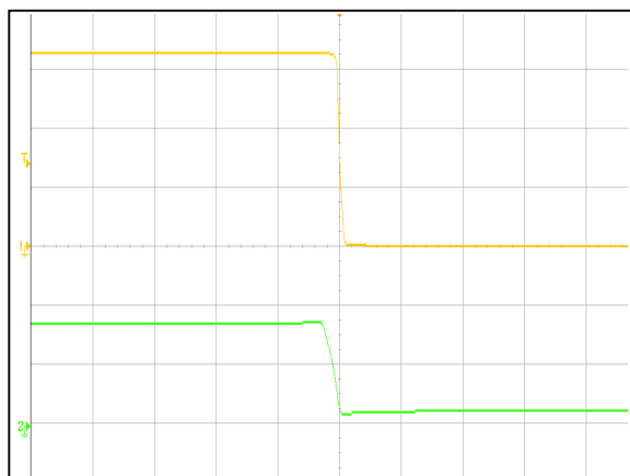
Figure 4: AVO100-36S3V3B-6L Turn Off Characteristic (2ms/div)
