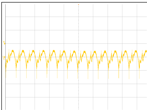
Figure 1: AVO100-36S3V3B-6L Ripple and Noise Measurement
