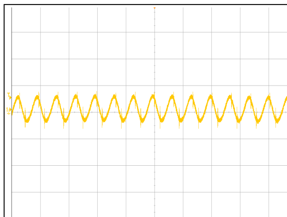
Figure 2: AVO100-36S3V3B-6L Input reflected ripple current
