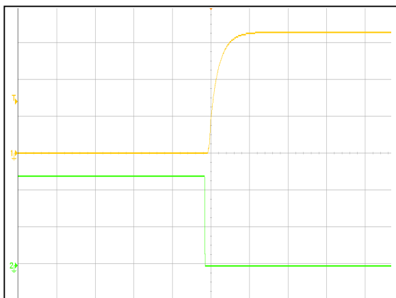
Figure 5: AVO100-36S3V3B-6L Remote ON Waveform (100ms/div)
