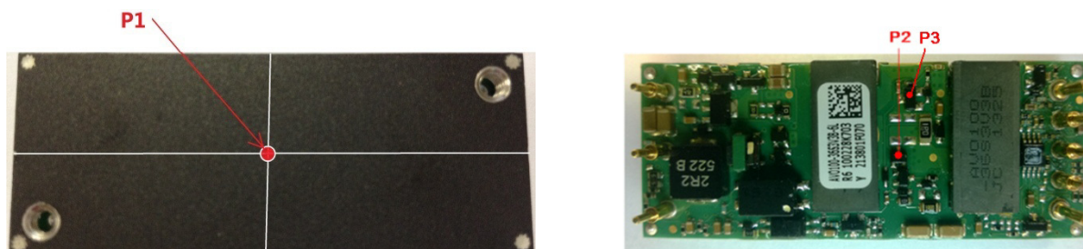
Figure 12 Temperature test point
