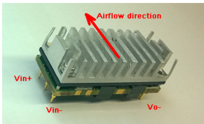
Figure 13 Typical test condition, heatsink size (L*W*H): 57.9mm*22.86*12.7mm
